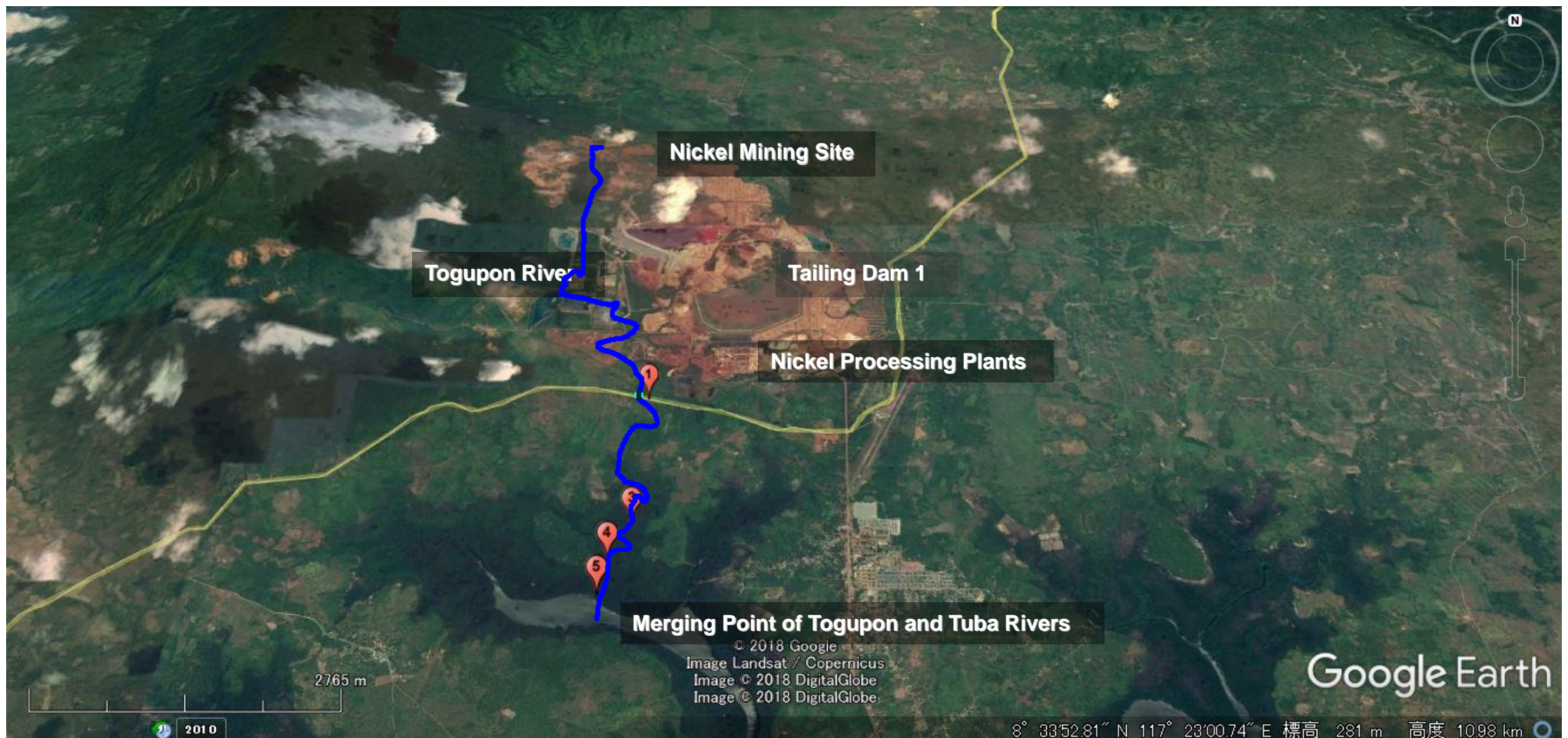
(Map) The Rio Tuba Nickel Mining site, the Coral Bay Nickel Processing Plants, the Togupon River, and Water Sampling points (April 29 and 30, 2018)
